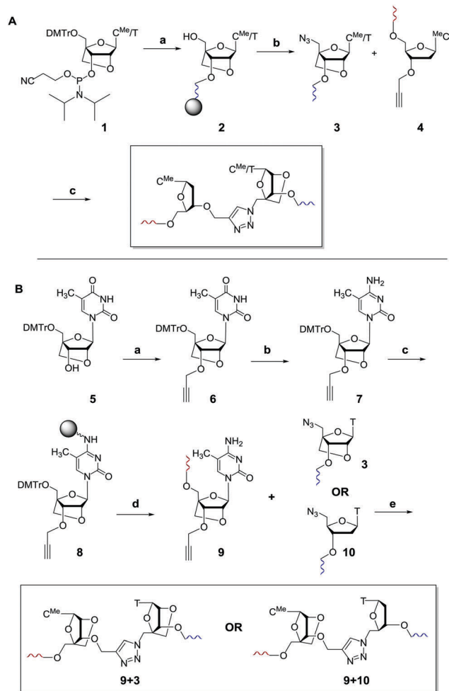
Scheme 1 (A) Synthesis of triazole 3'-LNA. (a) Automated solid phase DNA synthesis. (b) 1. Methyltriphenoxyphosphonium iodide, DMF; 2. \text{NaN}_3 , DMF, 55 °C; 3. aqueous ammonia, 55 °C. (c) \text{CuSO}_4 , sodium ascorbate, tris(3-hydroxypropyltriazolylmethyl)amine. 21 DMT = 5'-O-(4,4'-dimethoxytrityl), ^{\text{MeC}} = 5-methylcytosine. (B) Synthesis of triazole 5'-LNA and 5',3'-LNA. (a) 1. NaH, DMF, 0 °C, 30 min, rt, 1 h; 2. propargyl bromide, 0 °C, 30 min, rt, 16 h, 79%. (b) 1. N -Methylimidazole, 0 °C, 15 min; 2. \text{POCl}_3 , 0 °C, 30 min, rt, 30 min. 3. Conc. \text{NH}_3/\text{H}_2\text{O} , rt, 16 h, 57%. (c) 1. Amino resin, succinic anhydride, DMAP, pyridine, rt, 20 h; 2. DIC, HOBt, pyridine, rt, 20 h; 3. pentachlorophenol, pyridine, rt, 3 h; 4. piperidine (10% in DMF), rt, 5 min; 5. capping with acetic anhydride, N -methylimidazole 1:1, rt, 1 h to give 26 \mu\text{mol g}^{-1} loading of nucleoside on resin. (d) Automated solid phase DNA synthesis. (e) \text{CuSO}_4 , sodium ascorbate, tris(3-hydroxypropyltriazolylmethyl)amine. 21
